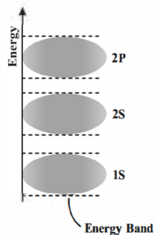
Figure 21.8 energy Bands
