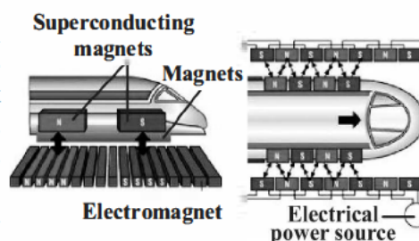
Figure 21.14 Magnetic Levitation
